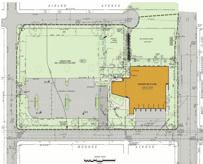
Site Layout
